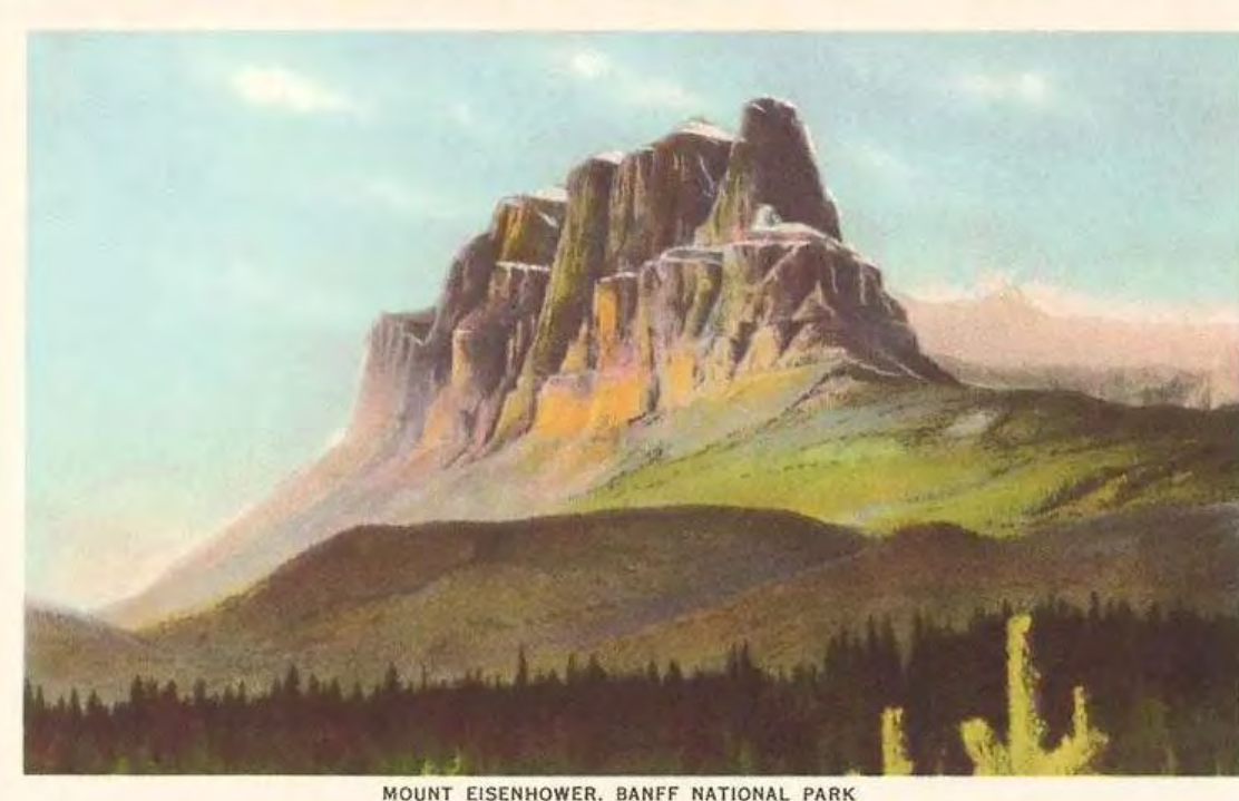
MOUNT EISENHOWER, BANFF NATIONAL PARK
