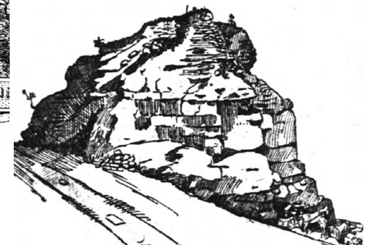
ALL THAT'S LEFT OF THE MOUNTAIN.
